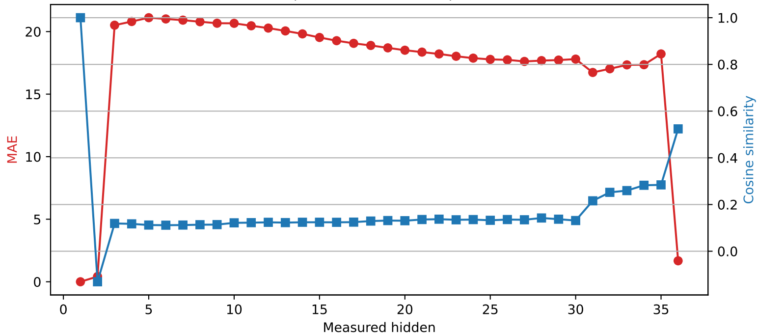
Qwen2.5-3B | Quantized layer 1 | float16 → int2
