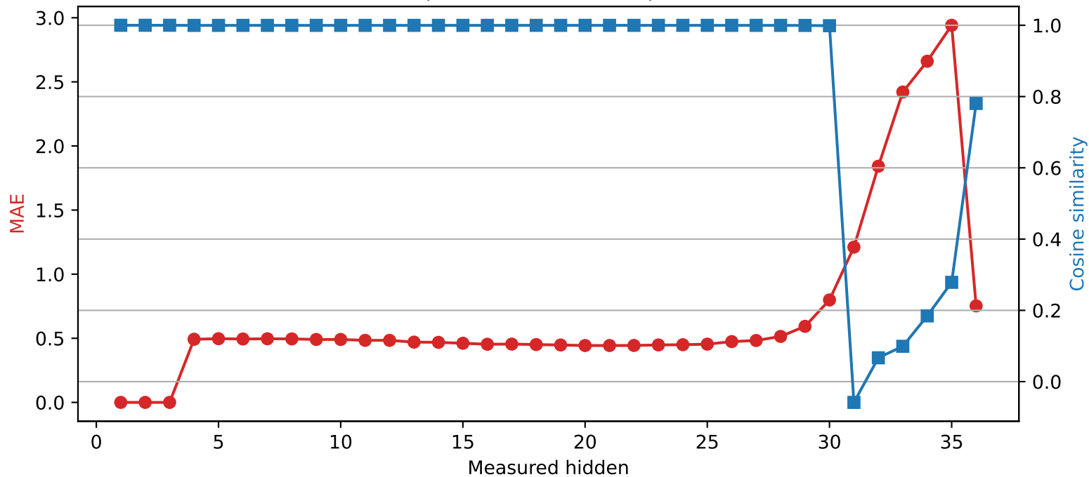
Qwen2.5-3B | Quantized layer 3 | float16 \rightarrow int2
