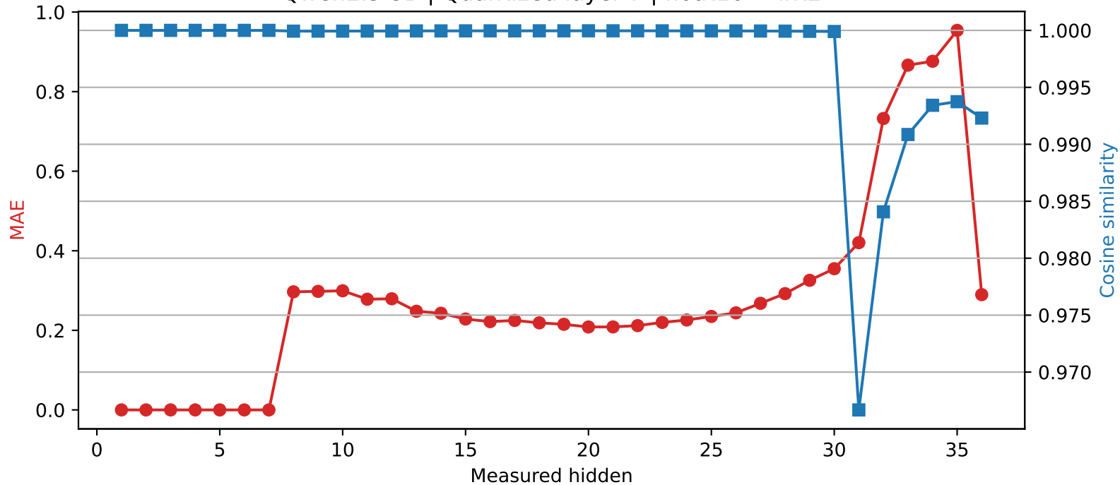
Qwen2.5-3B | Quantized layer 7 | float16 → int2
