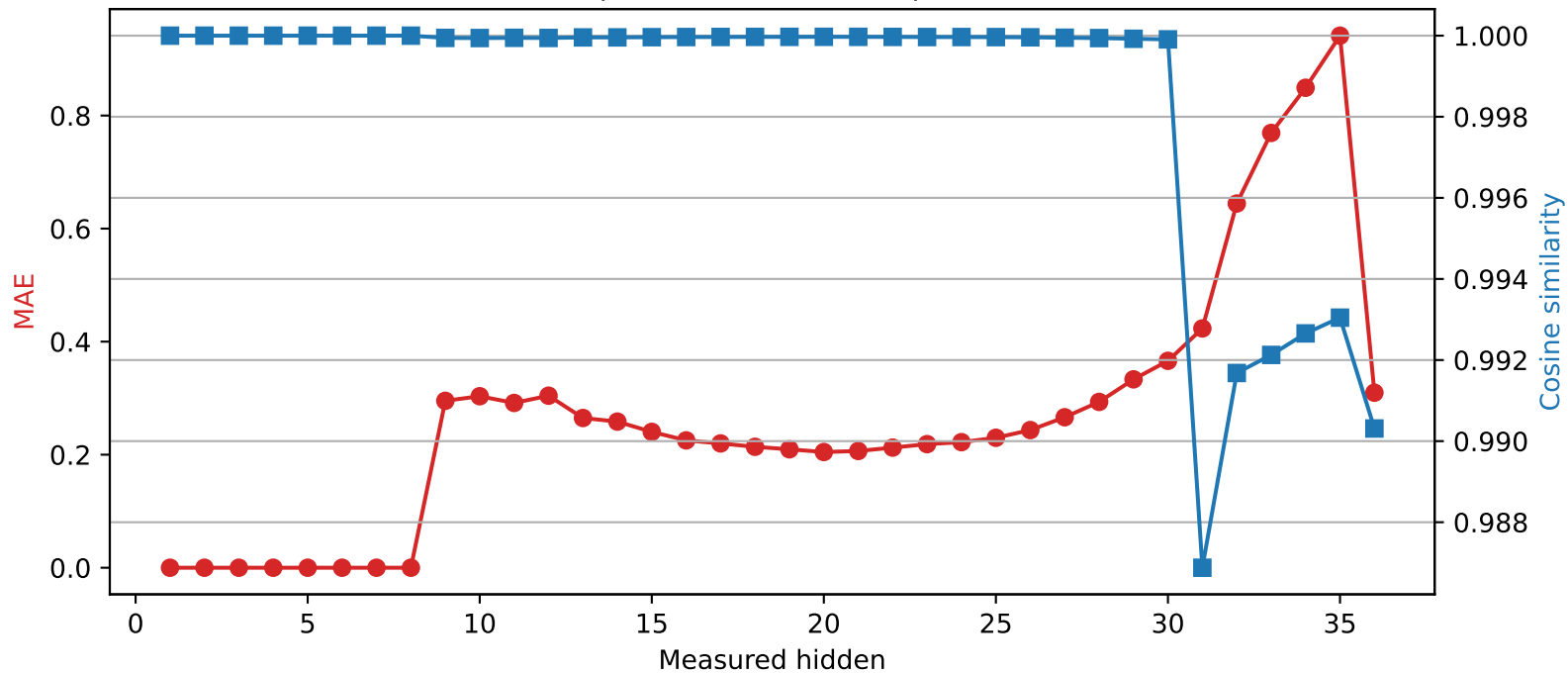
Qwen2.5-3B | Quantized layer 8 | float16 → int2
