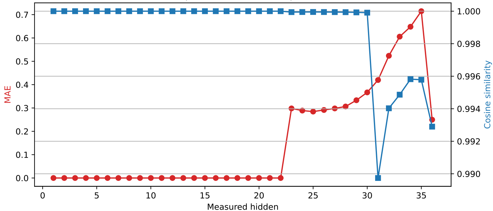
Qwen2.5-3B | Quantized layer 22 | float16 → int2
