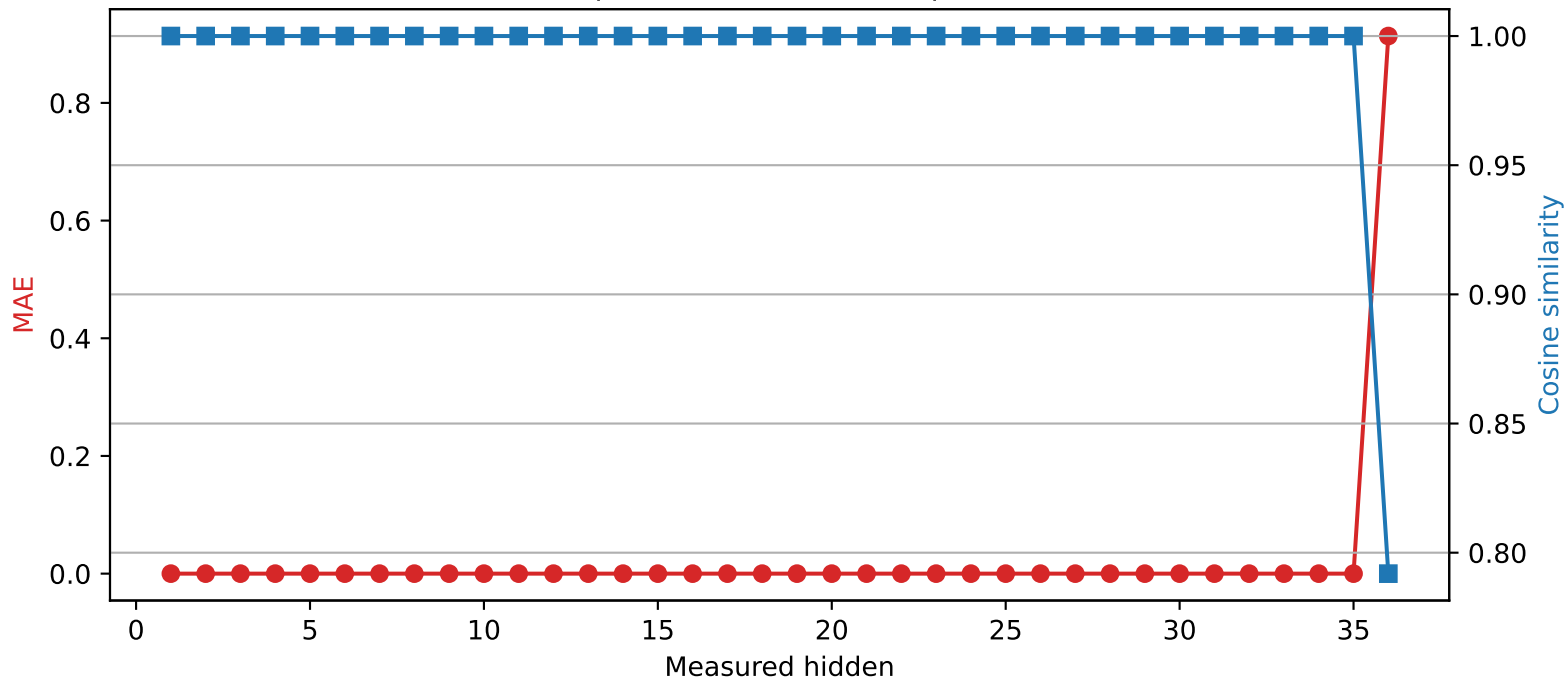
Qwen2.5-3B | Quantized layer 35 | float16 \rightarrow int2
