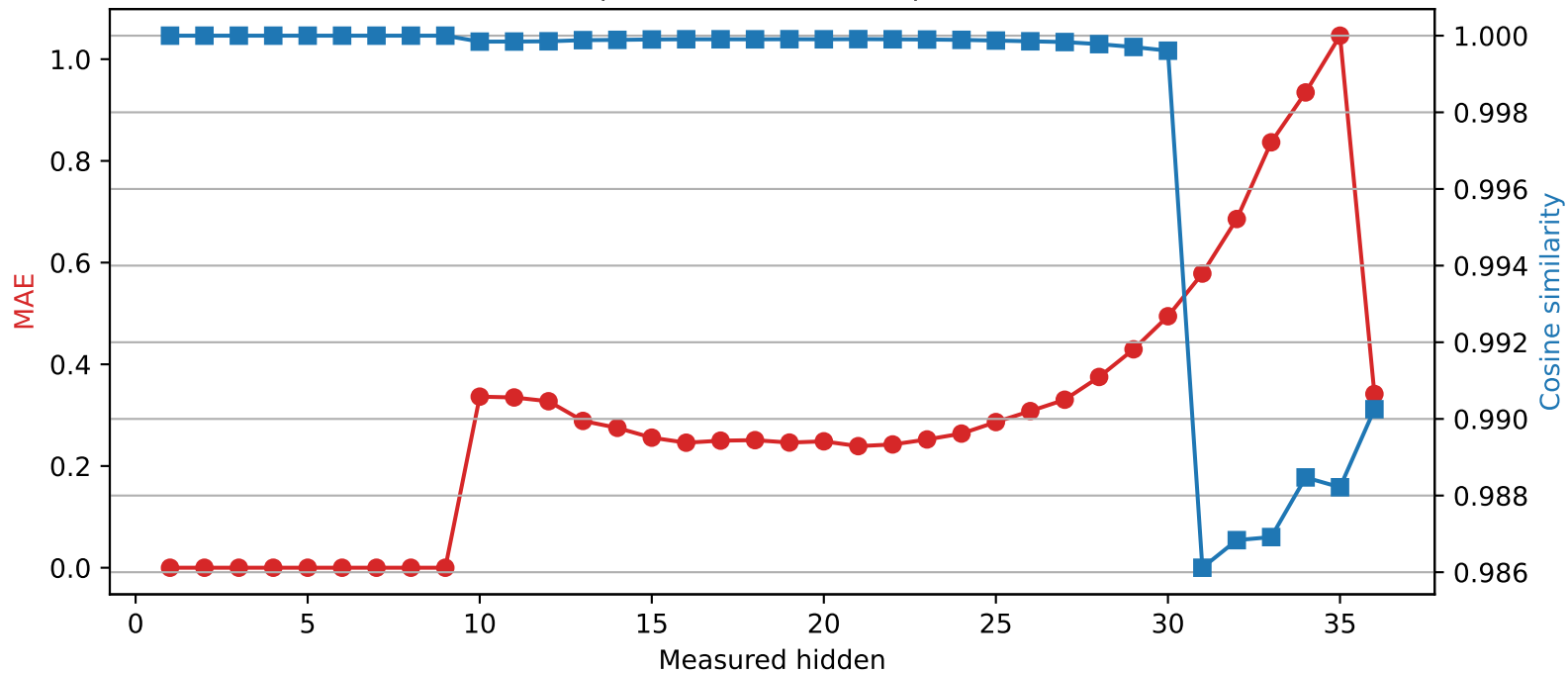
Qwen2.5-3B | Quantized layer 9 | float16 \rightarrow int2
