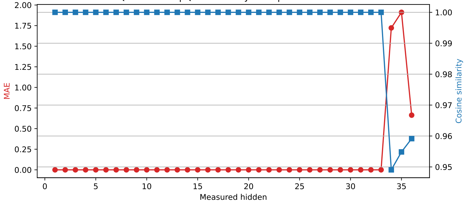
Qwen2.5-3B | Quantized layer 33 | float16 → int2
