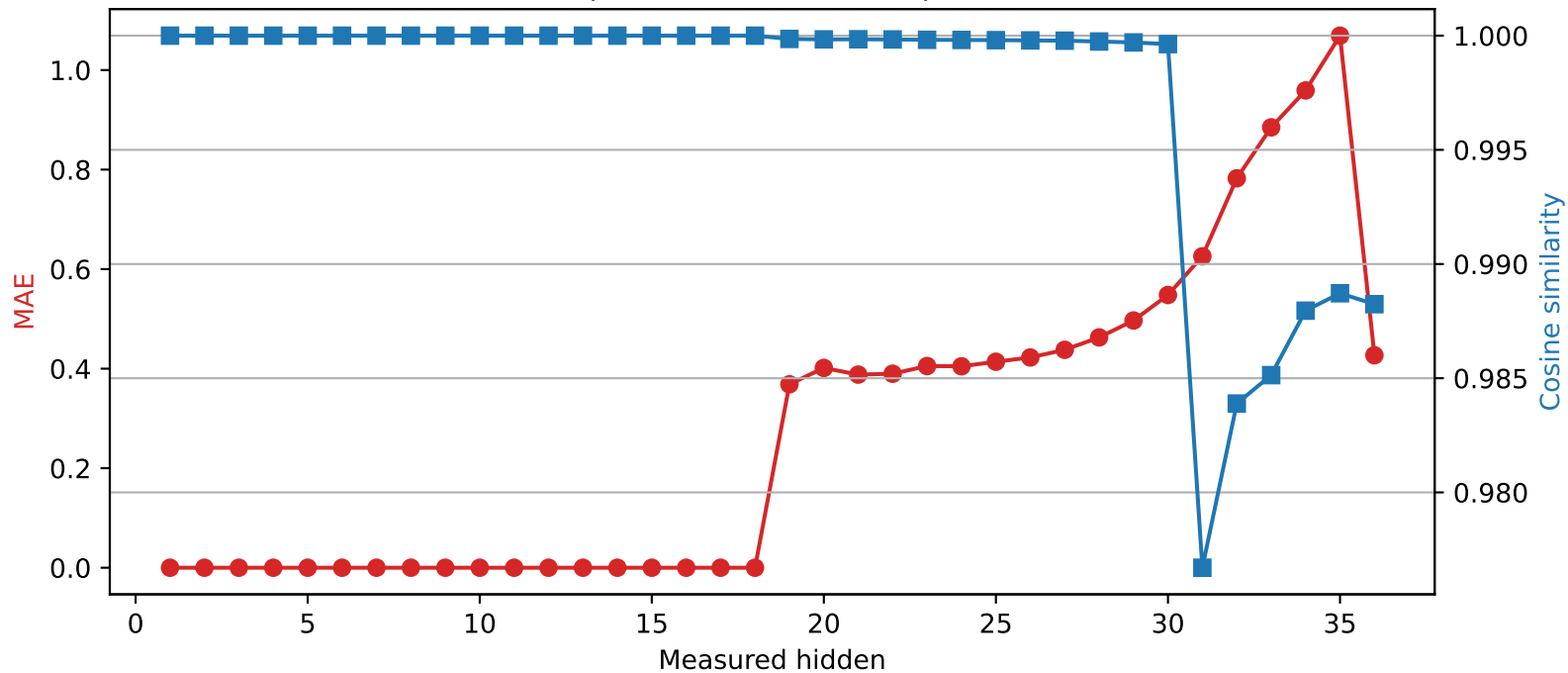
Qwen2.5-3B | Quantized layer 18 | float16 → int2
