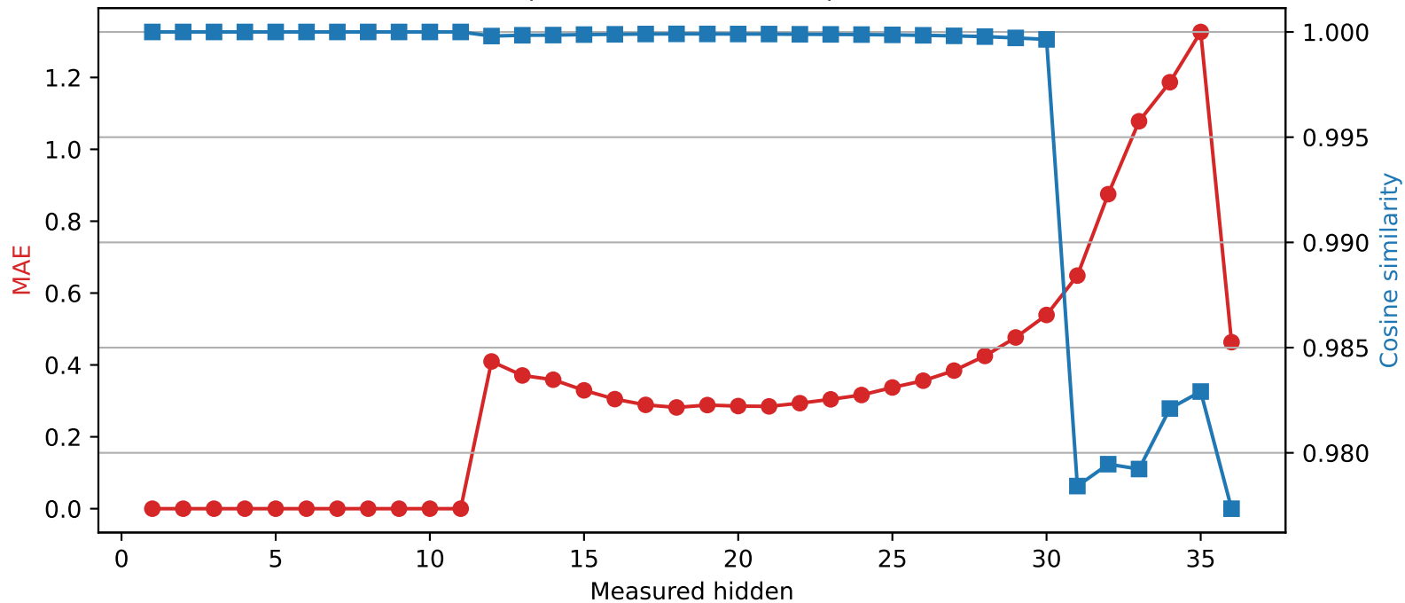
Qwen2.5-3B | Quantized layer 11 | float16 \rightarrow int2
