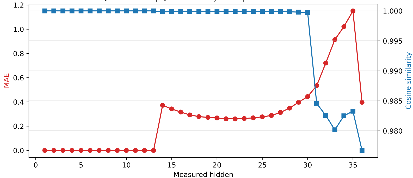
Qwen2.5-3B | Quantized layer 13 | float16 \rightarrow int2
