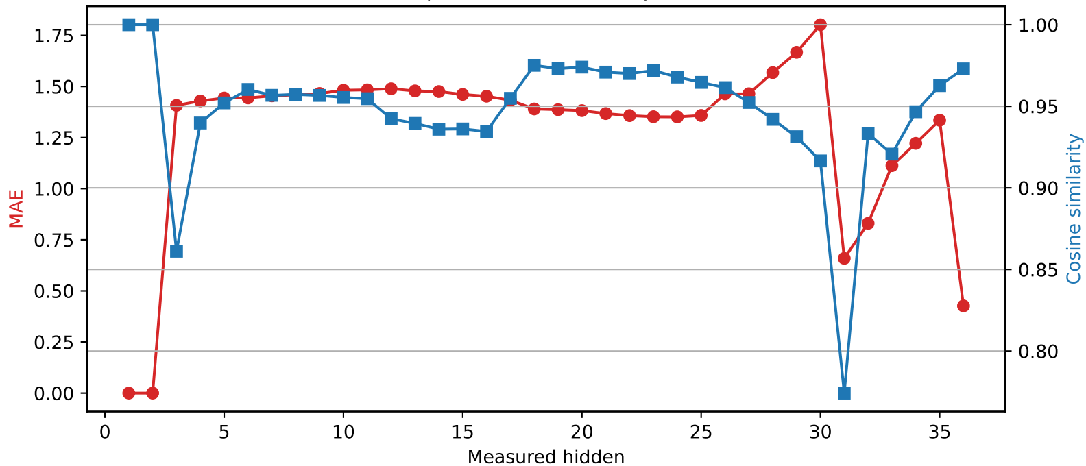
Qwen2.5-3B | Quantized layer 2 | float16 \rightarrow int2
