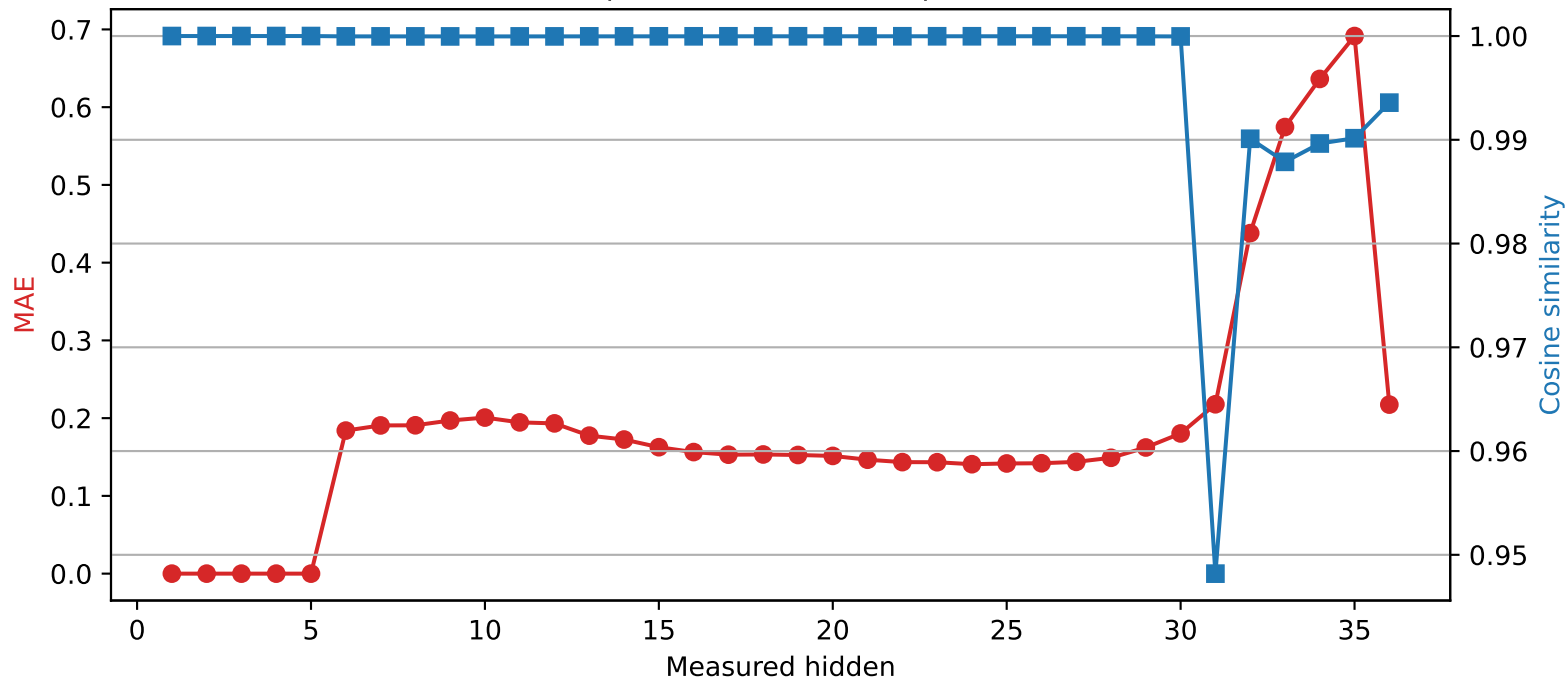
Qwen2.5-3B | Quantized layer 5 | float16 \rightarrow int2
