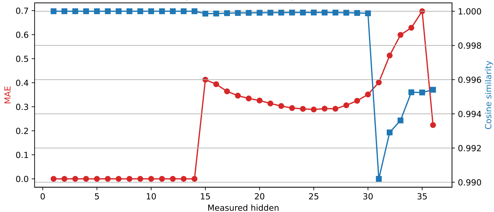
Qwen2.5-3B | Quantized layer 14 | float16 → int2
