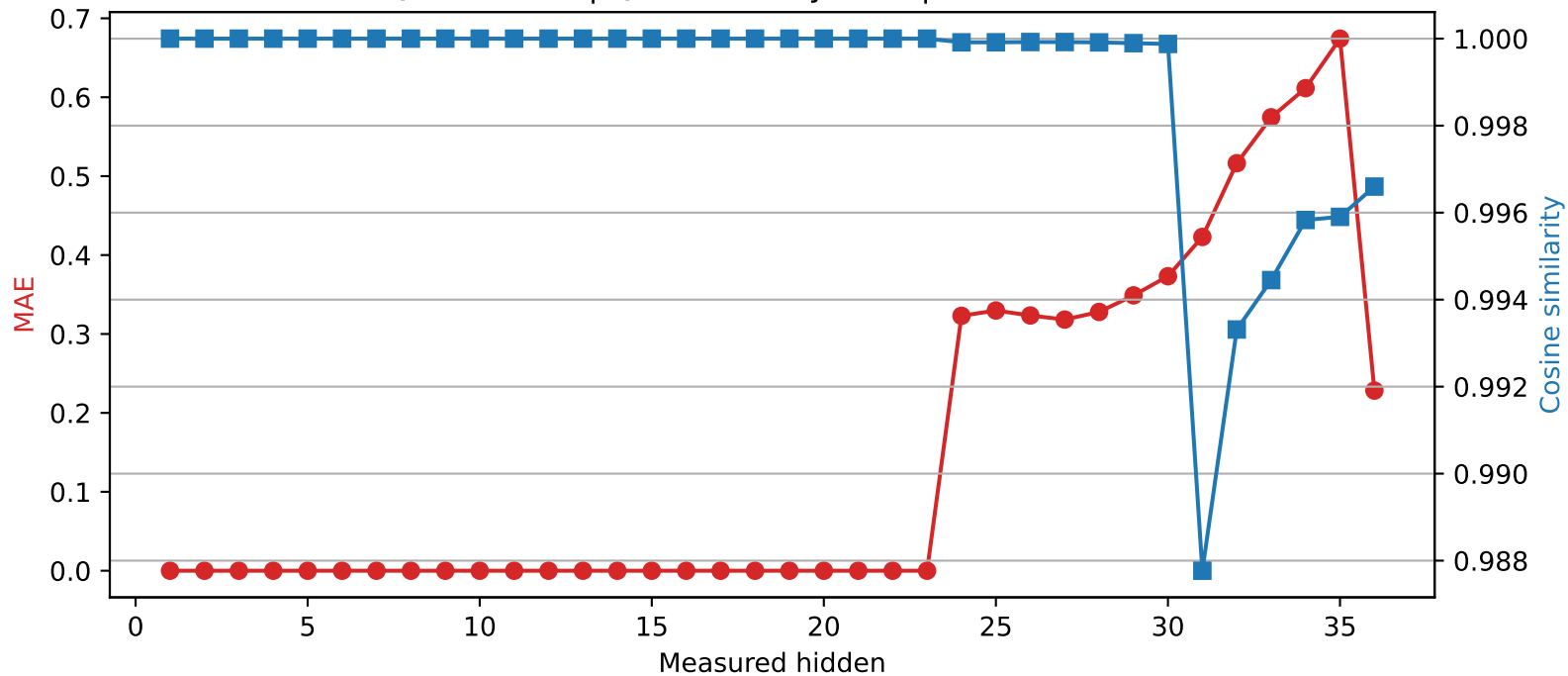
Qwen2.5-3B | Quantized layer 23 | float16 → int2
