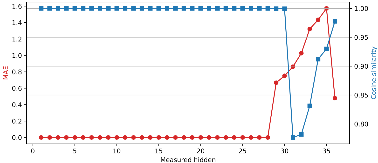
Qwen2.5-3B | Quantized layer 28 | float16 → int2
