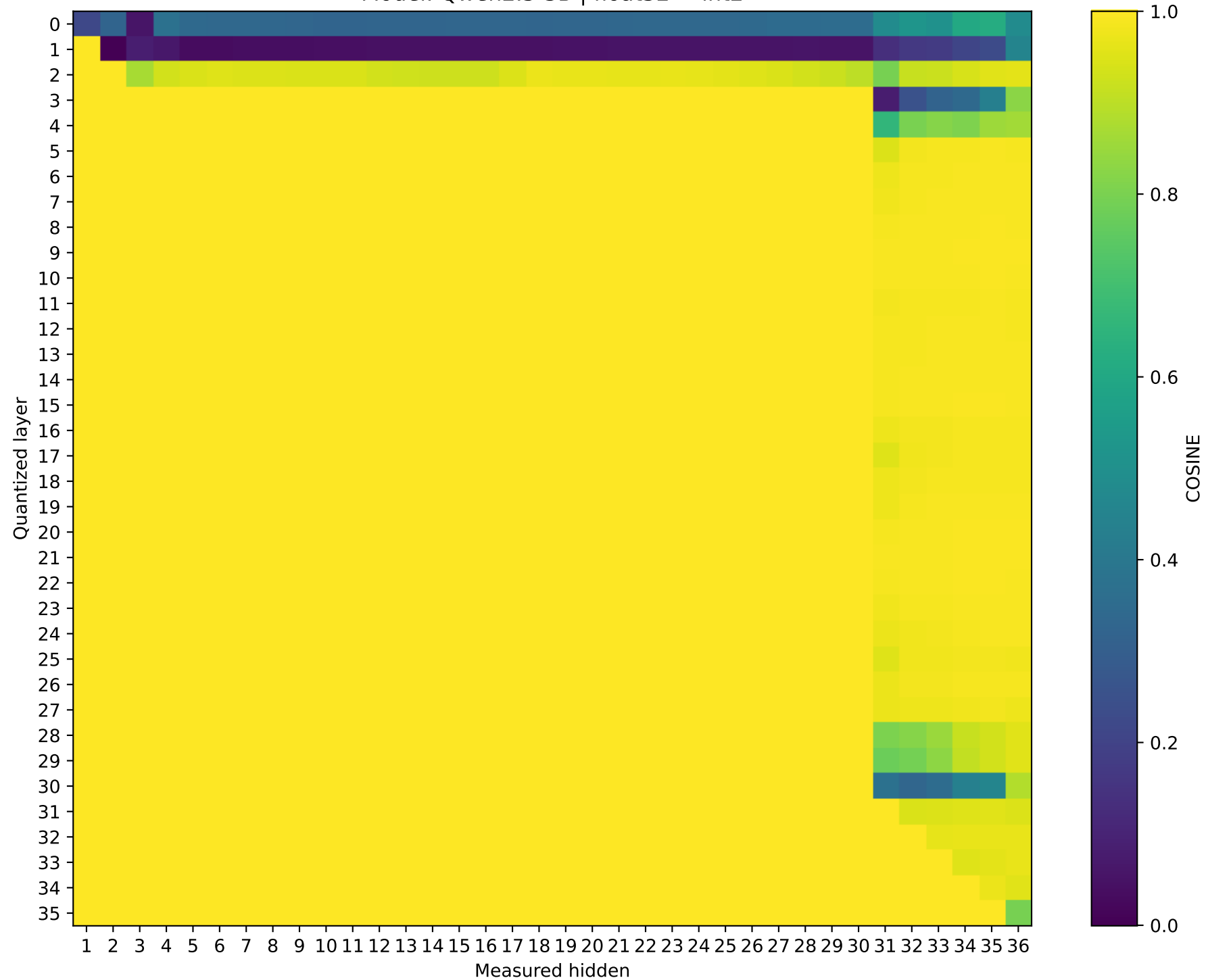
Model: Qwen2.5-3B | float32 \rightarrow int2
