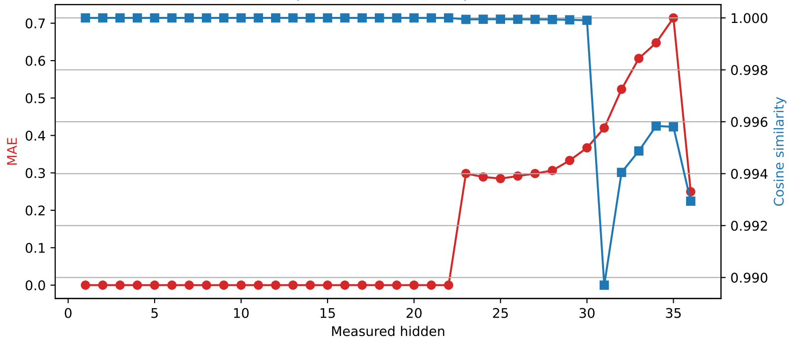
Qwen2.5-3B | Quantized layer 22 | float32 → int2
