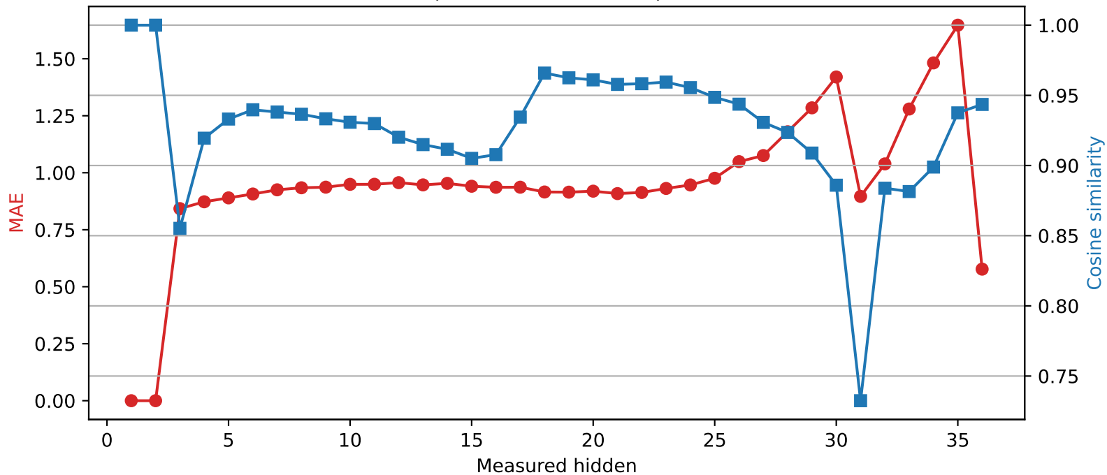
Qwen2.5-3B | Quantized layer 2 | float32 → int2
