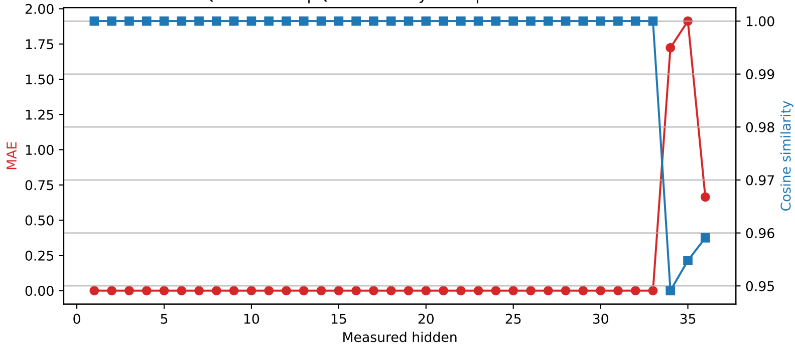
Qwen2.5-3B | Quantized layer 33 | float32 → int2
