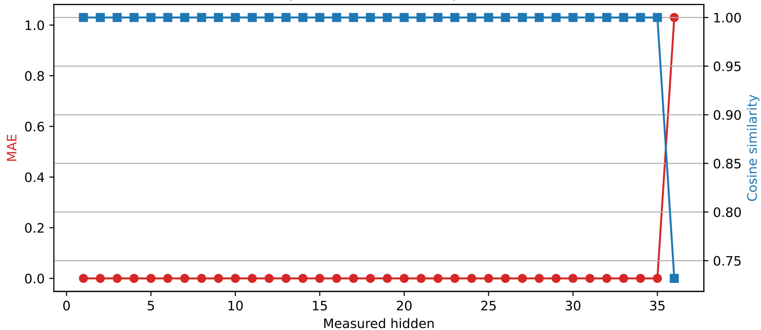
Qwen2.5-3B | Quantized layer 35 | float32 \rightarrow int2
