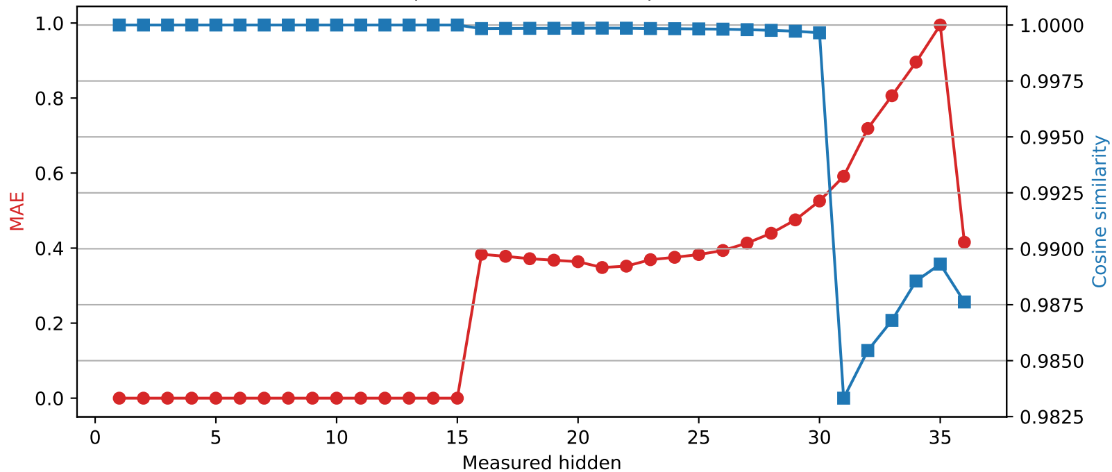
Qwen2.5-3B | Quantized layer 15 | float32 → int2
