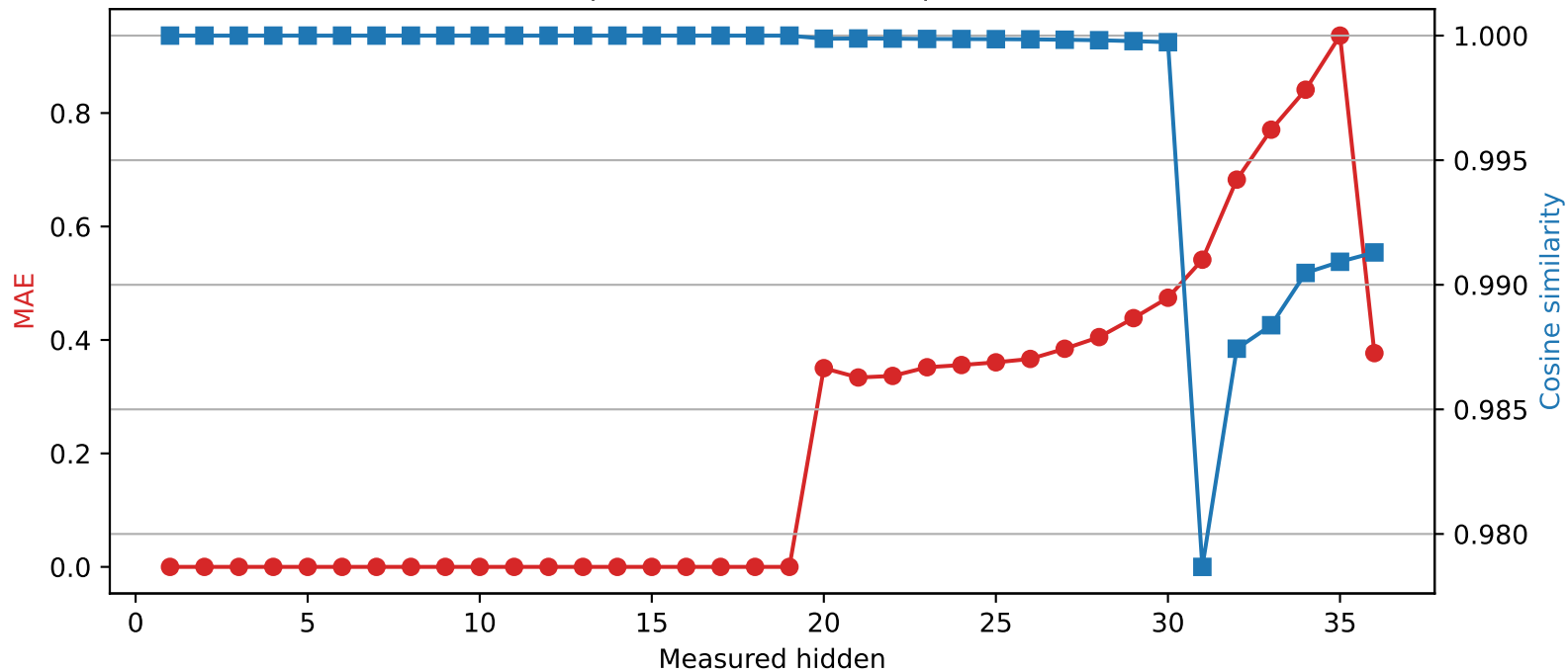
Qwen2.5-3B | Quantized layer 19 | float32 → int2
