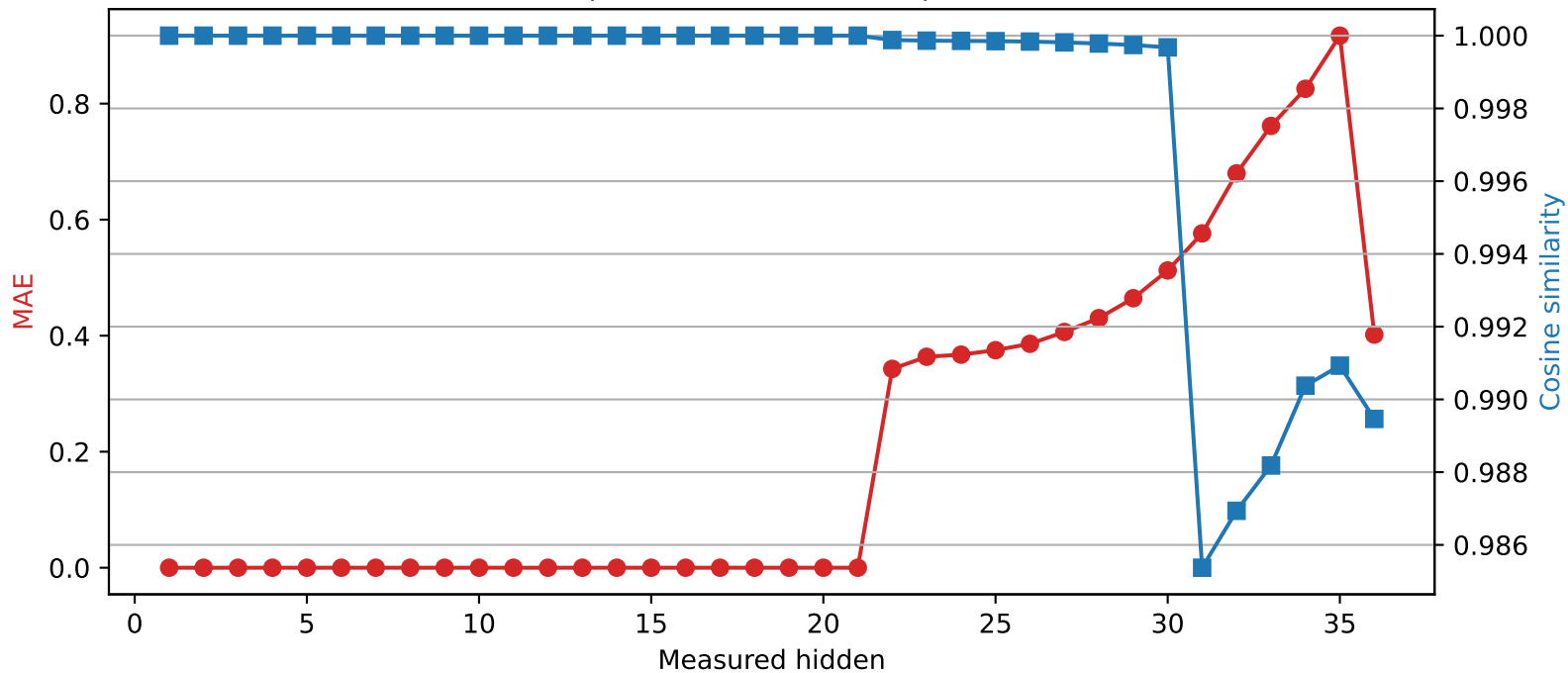
Qwen2.5-3B | Quantized layer 21 | float32 → int2
