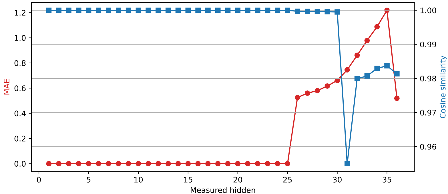
Qwen2.5-3B | Quantized layer 25 | float32 → int2
