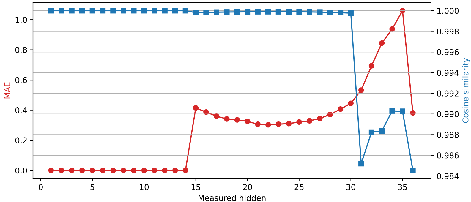
Qwen2.5-3B | Quantized layer 14 | float32 → int2
