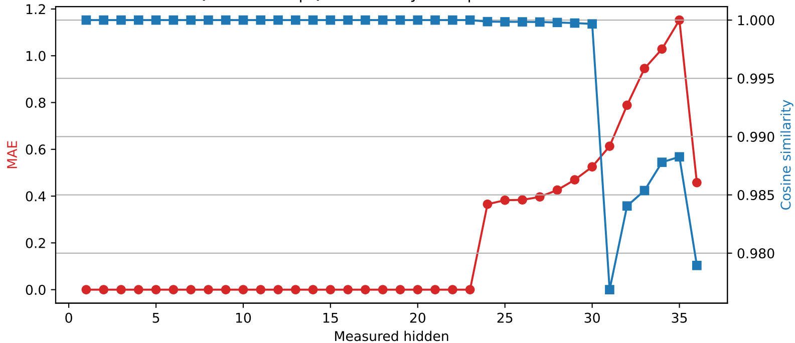
Qwen2.5-3B | Quantized layer 23 | float32 → int2
