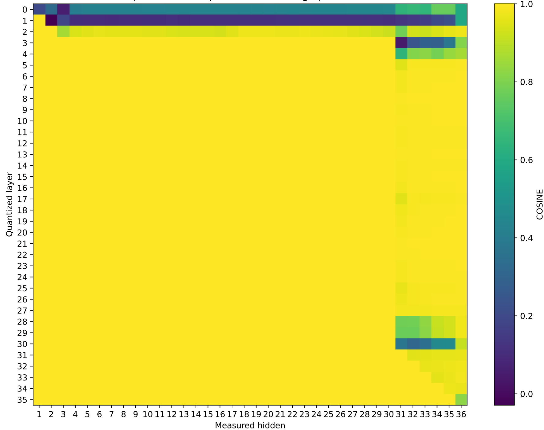
Qwen2.5-3B Prompt 4: cos sim representation damage | float32 → int2
