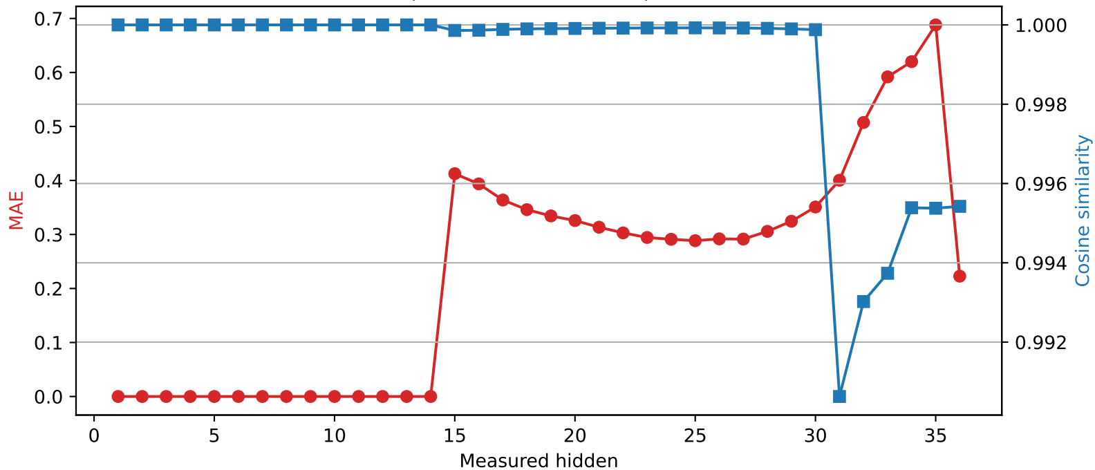
Qwen2.5-3B | Quantized layer 14 | float32 \rightarrow int2
