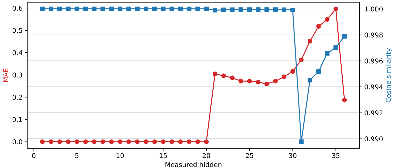
Qwen2.5-3B | Quantized layer 20 | float32 → int2
