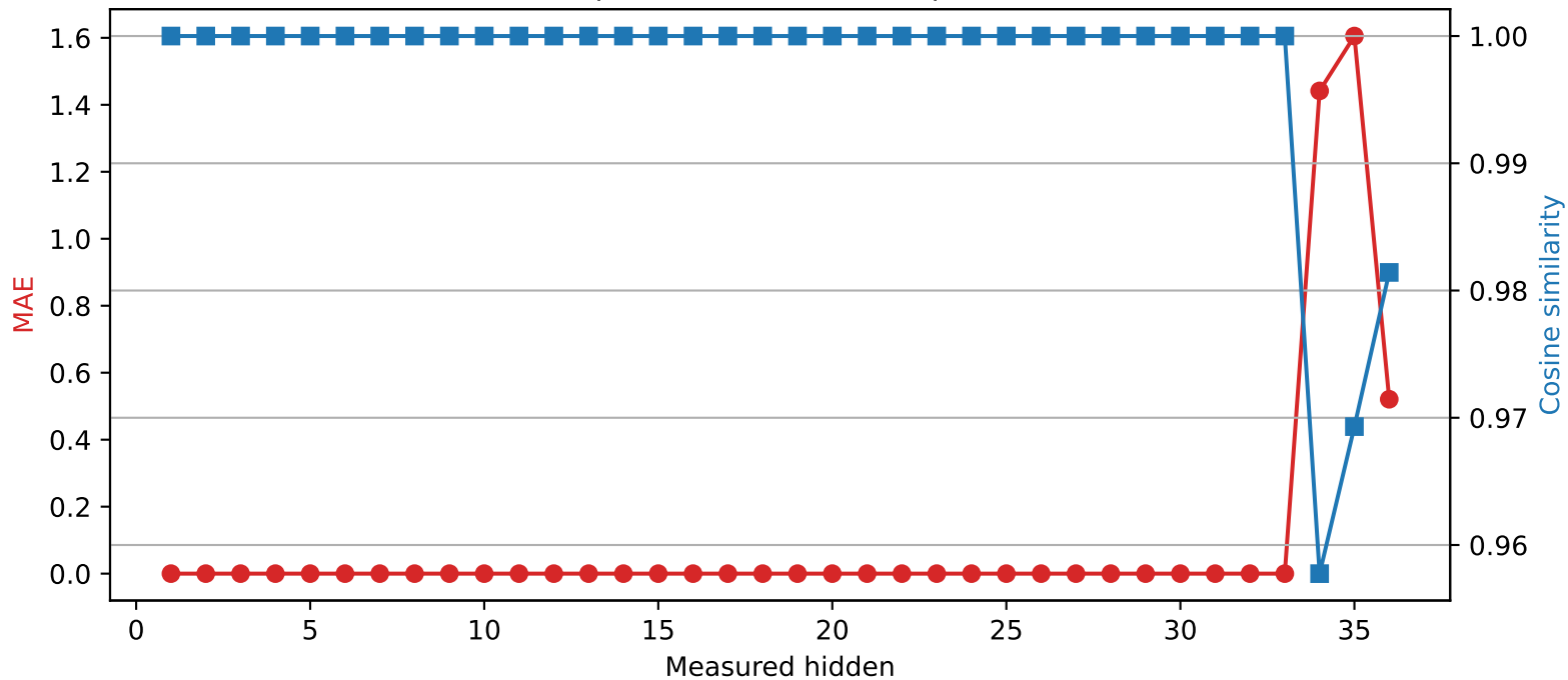
Qwen2.5-3B | Quantized layer 33 | float32 \rightarrow int2
