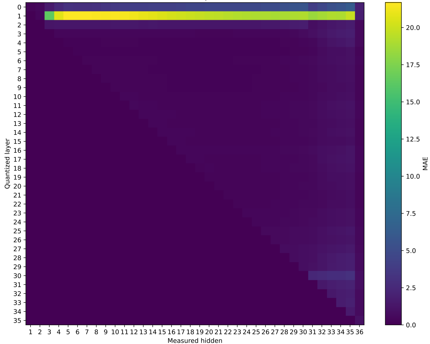
Model: Qwen2.5-3B | float64 → int2
