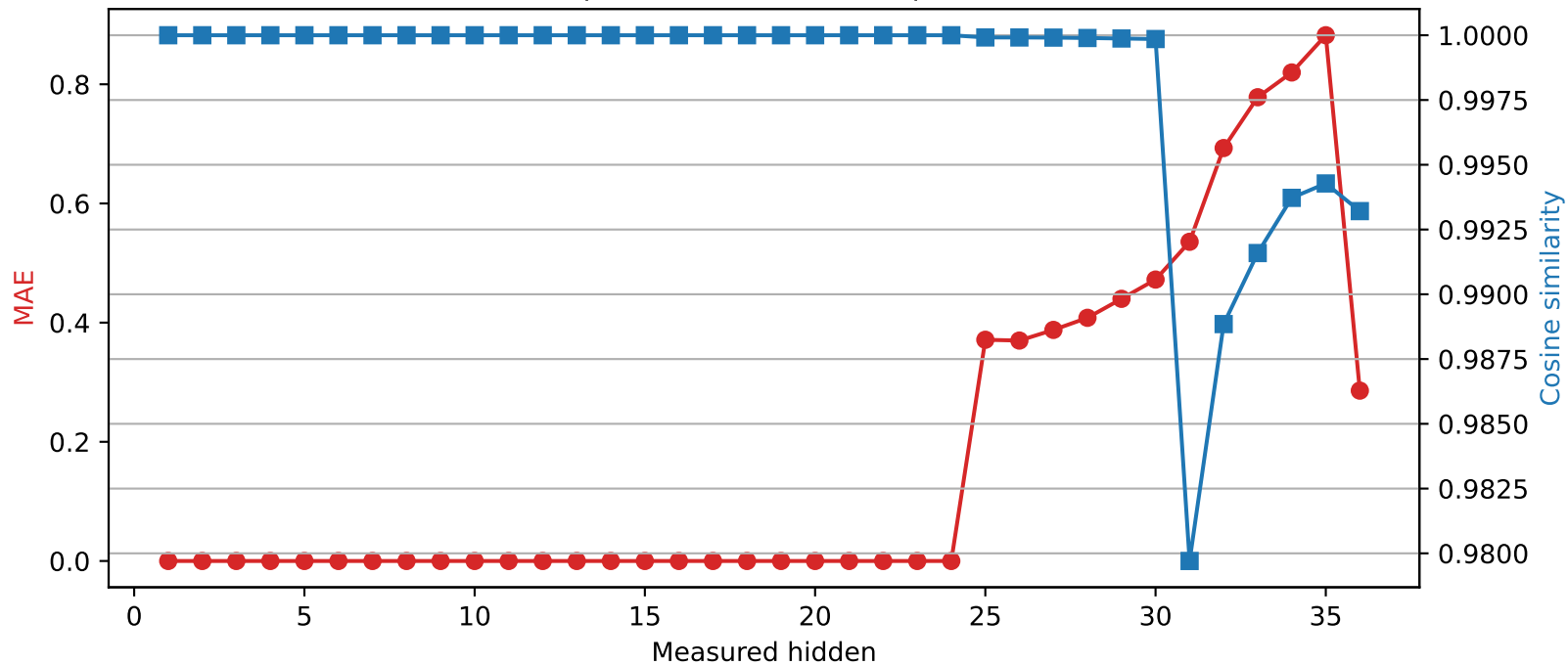
Qwen2.5-3B | Quantized layer 24 | float64 → int2
