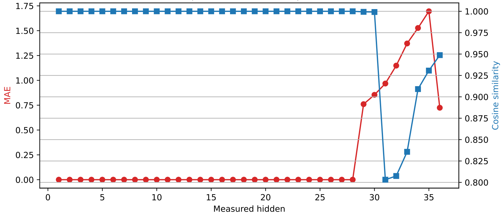
Qwen2.5-3B | Quantized layer 28 | float64 → int2
