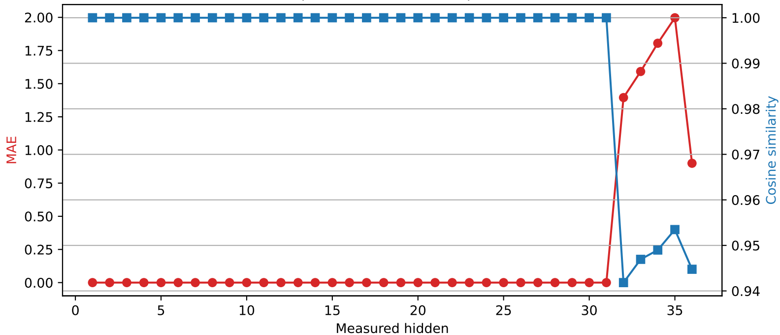
Qwen2.5-3B | Quantized layer 31 | float64 → int2
