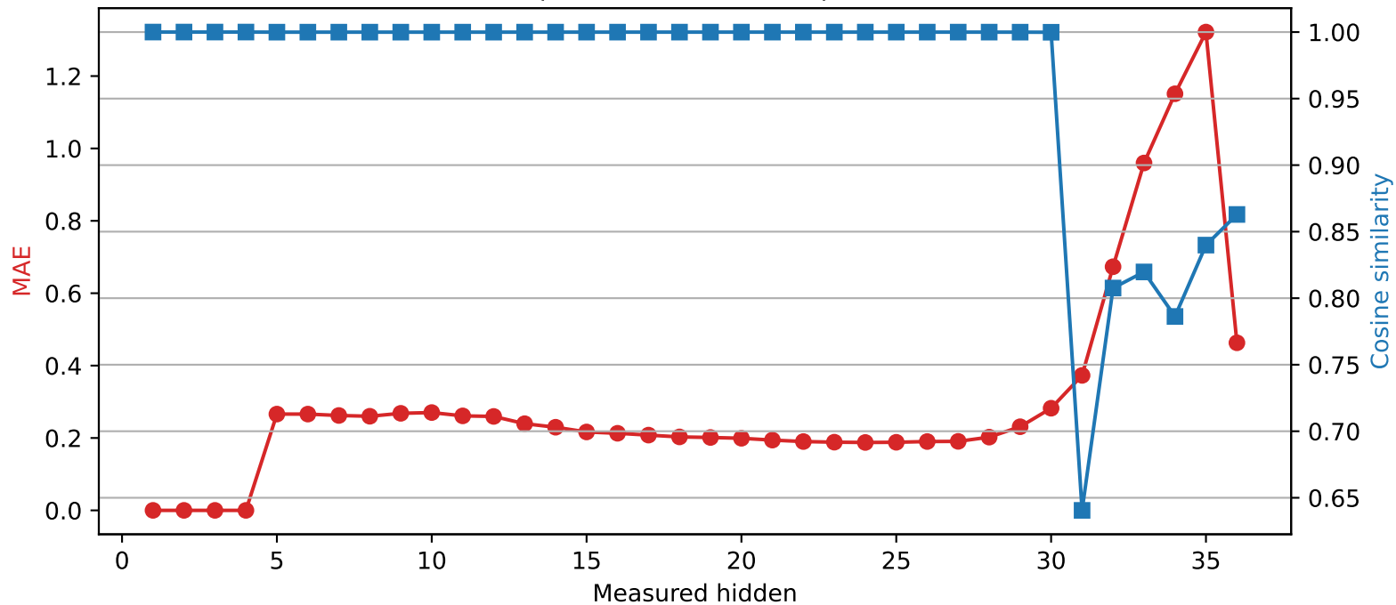
Qwen2.5-3B | Quantized layer 4 | float64 → int2
