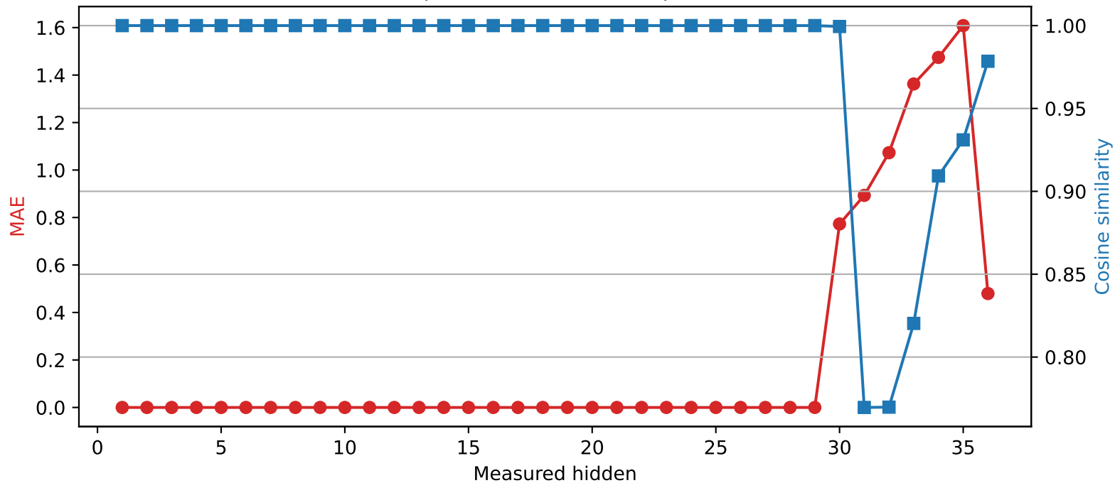
Qwen2.5-3B | Quantized layer 29 | float64 → int2
