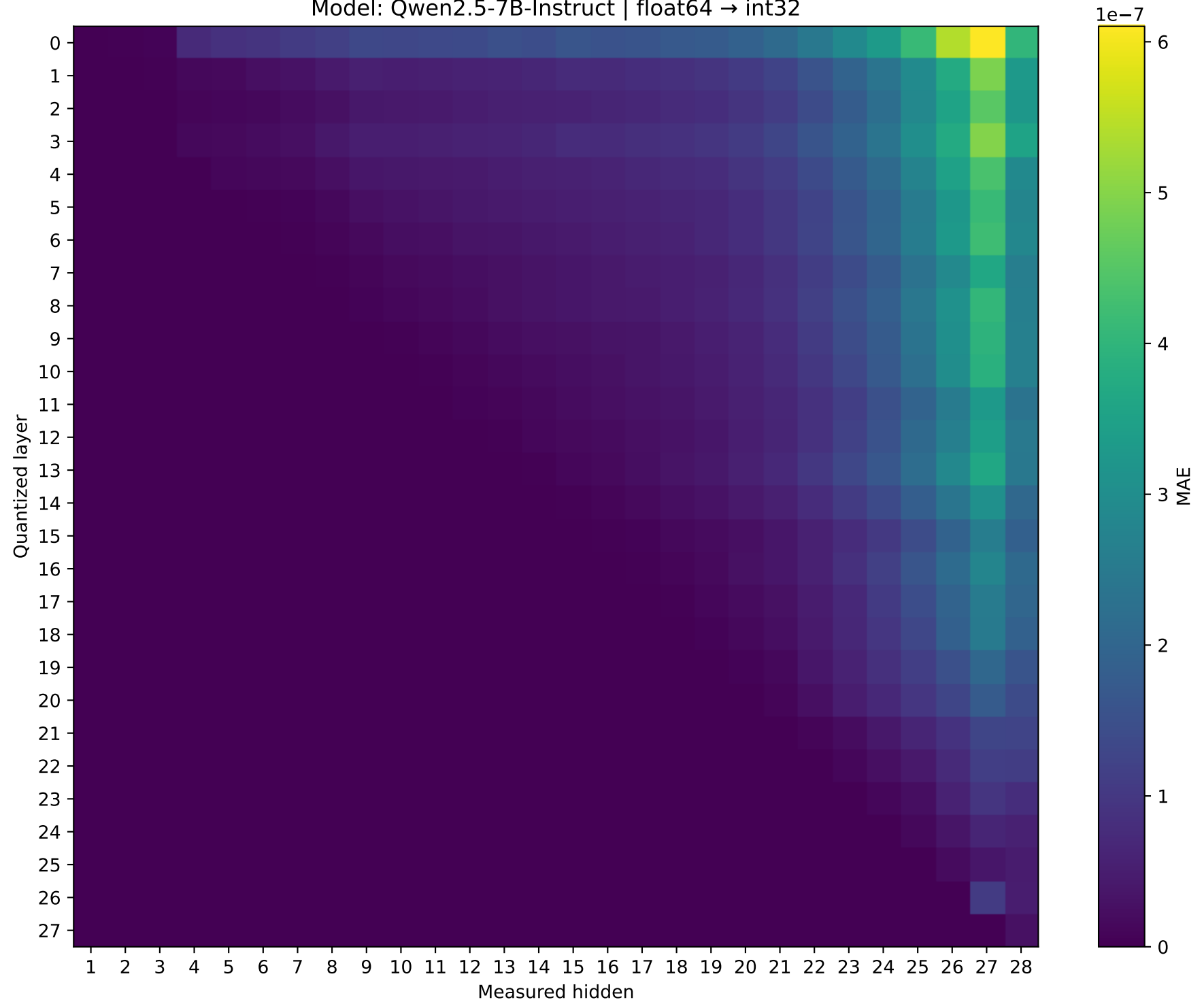
Model: Qwen2.5-7B-Instruct | float64 → int32
