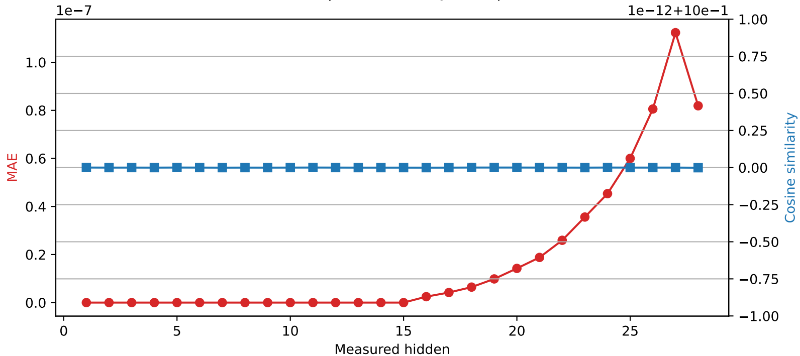
Qwen2.5-7B-Instruct | Quantized layer 15 | float64 → int32
