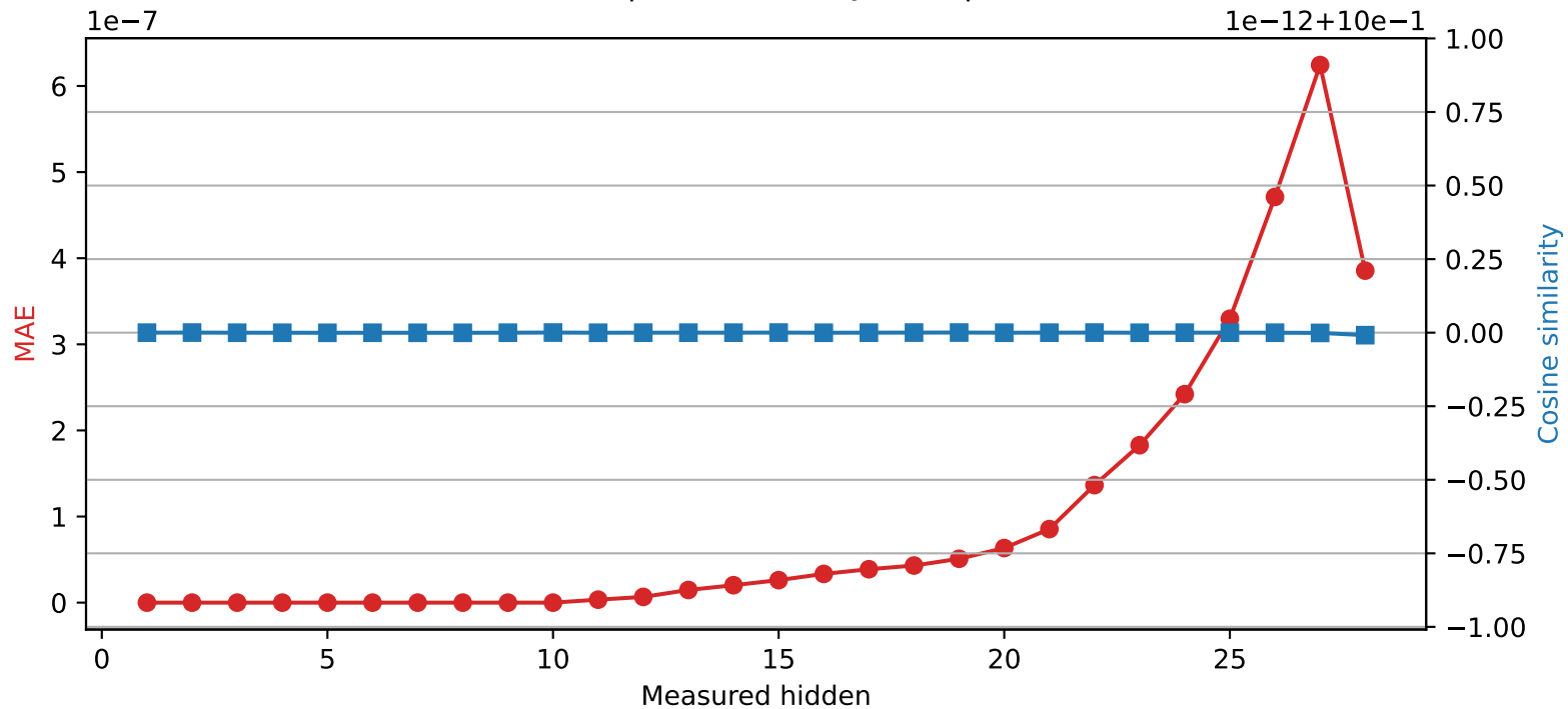
Qwen2.5-7B-Instruct | Quantized layer 10 | float64 → int32
