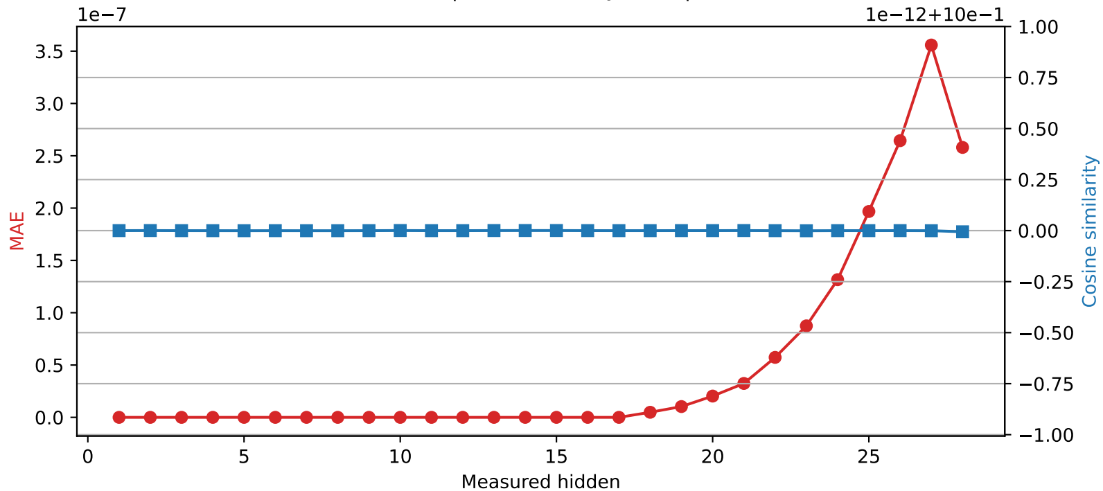
Qwen2.5-7B-Instruct | Quantized layer 17 | float64 → int32
