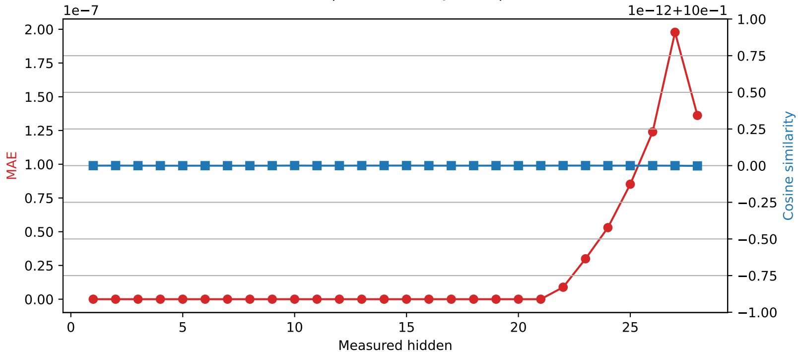
Qwen2.5-7B-Instruct | Quantized layer 21 | float64 → int32
