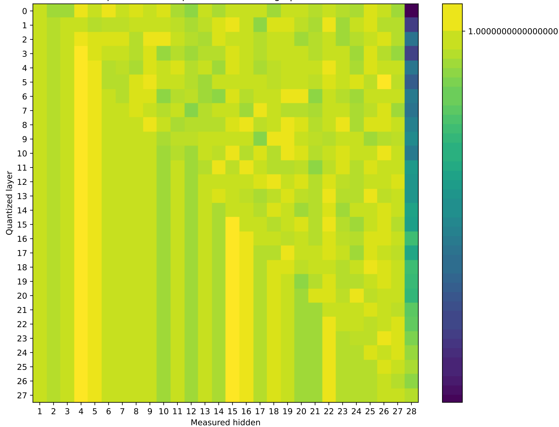
Qwen2.5-7B-Instruct Prompt 2: cos sim representation damage | float64 → int32
