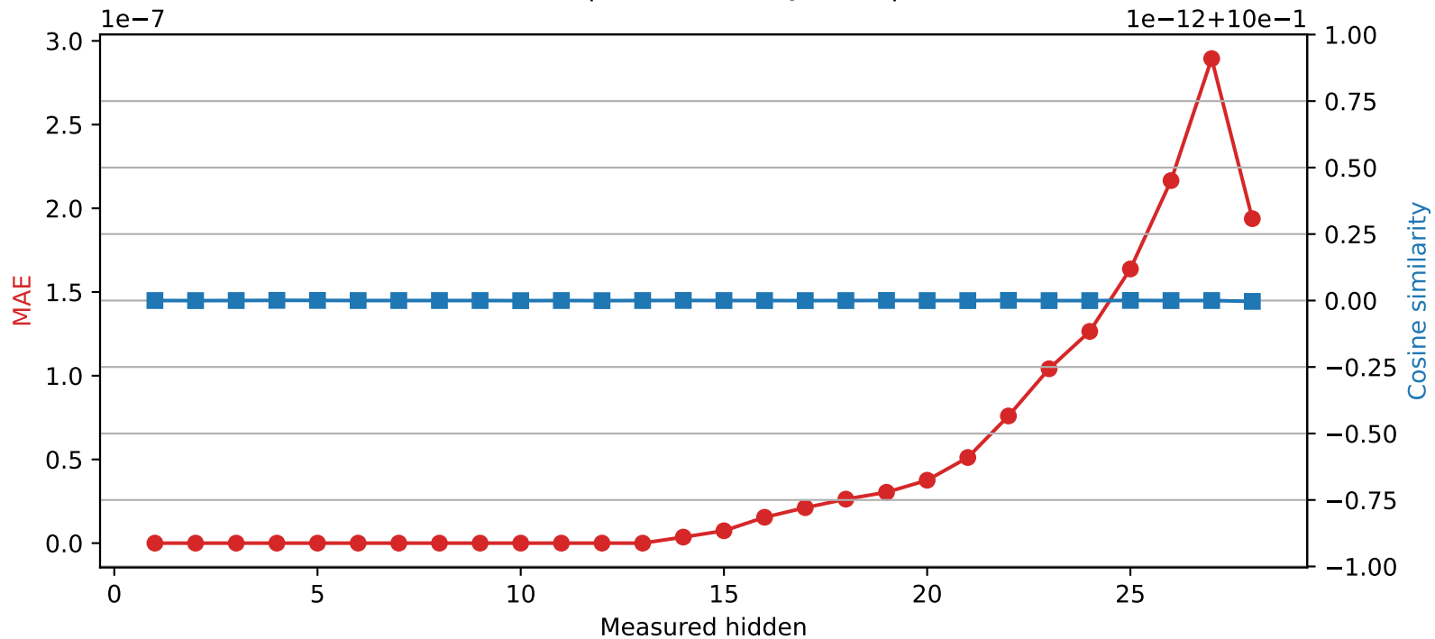
Qwen2.5-7B-Instruct | Quantized layer 13 | float64 → int32
