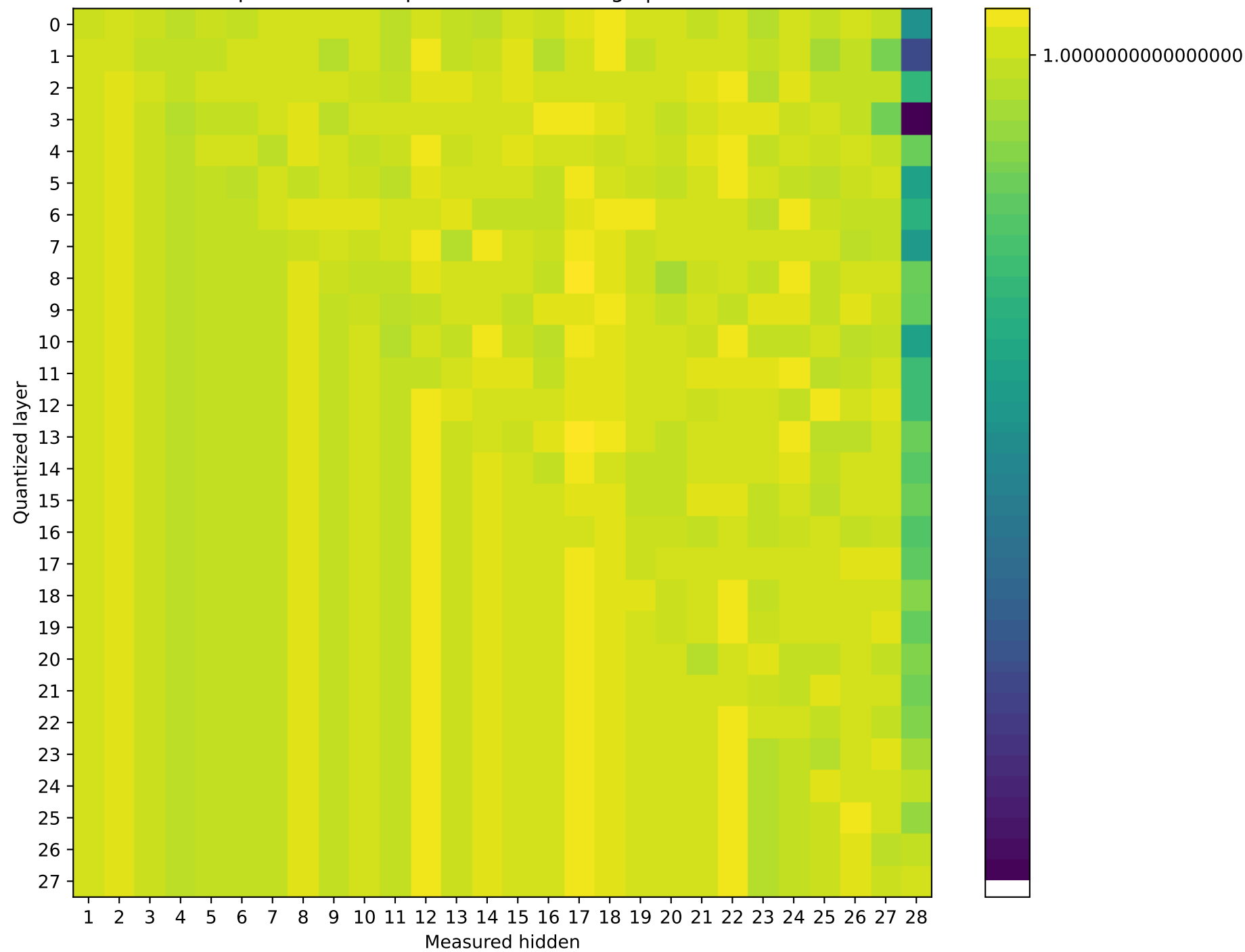
Qwen2.5-7B-Instruct Prompt 4: cos sim representation damage | float64 → int32
