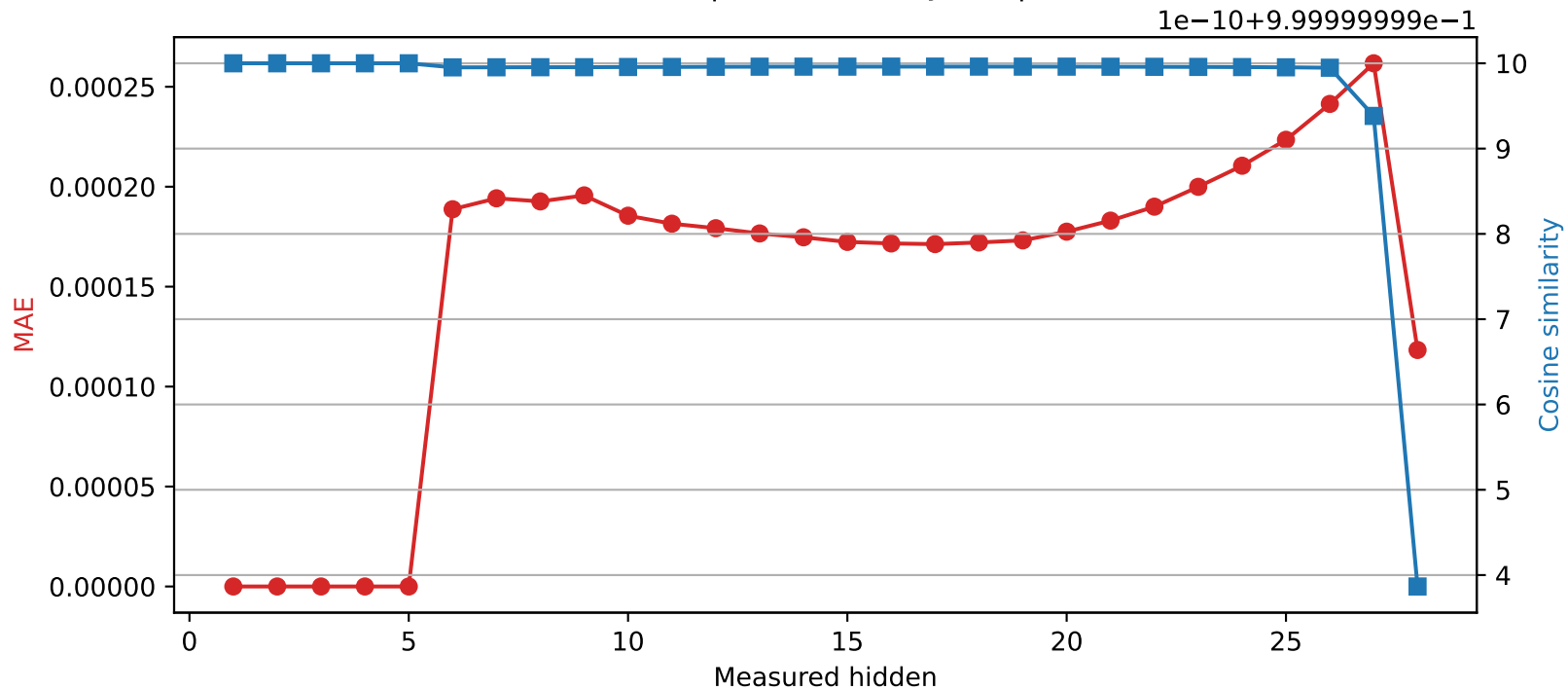
Qwen2.5-7B-Instruct | Quantized layer 5 | float32 \rightarrow int16
