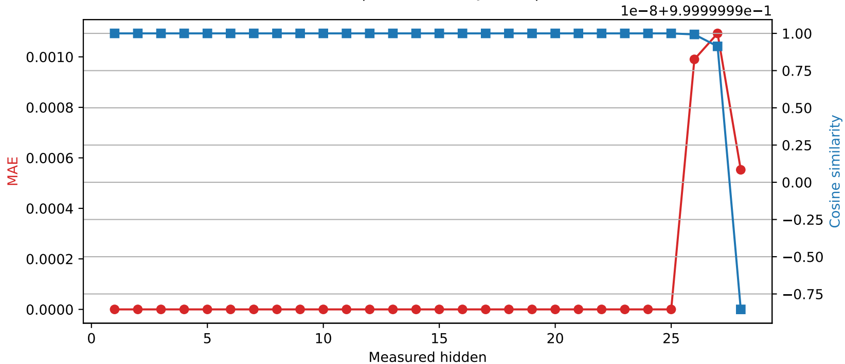
Qwen2.5-7B-Instruct | Quantized layer 25 | float32 \rightarrow int16
