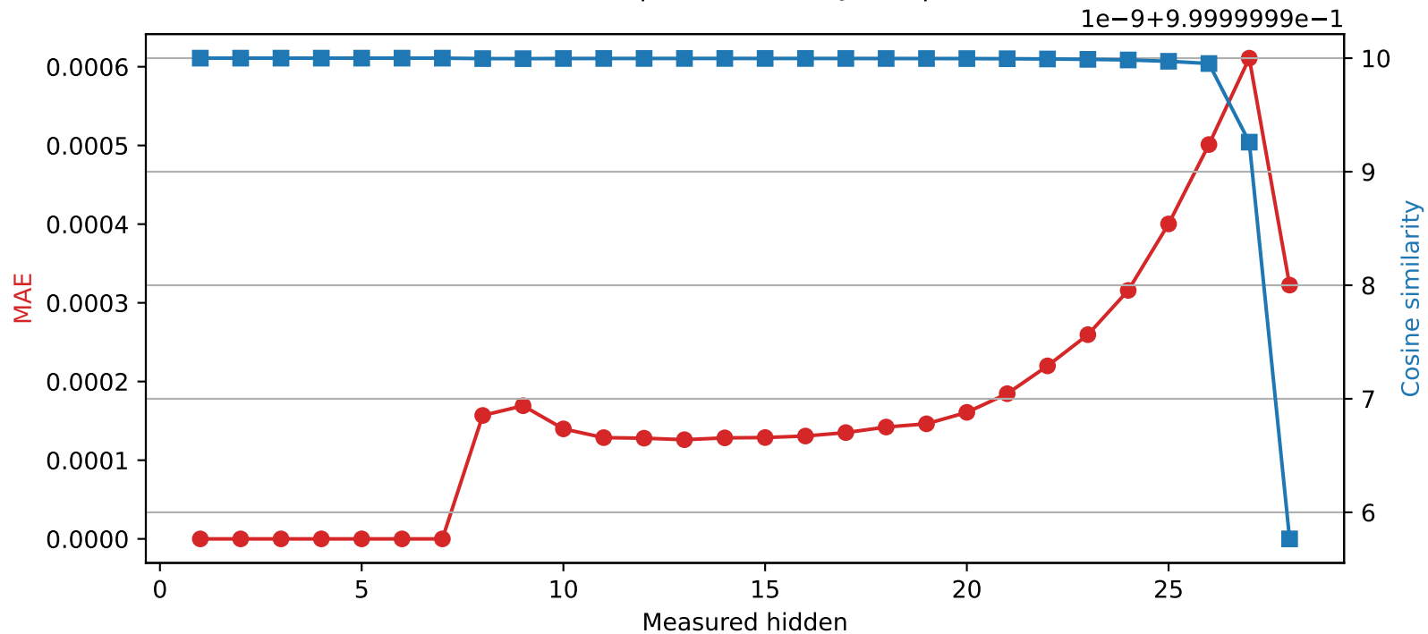
Qwen2.5-7B-Instruct | Quantized layer 7 | float32 → int16
