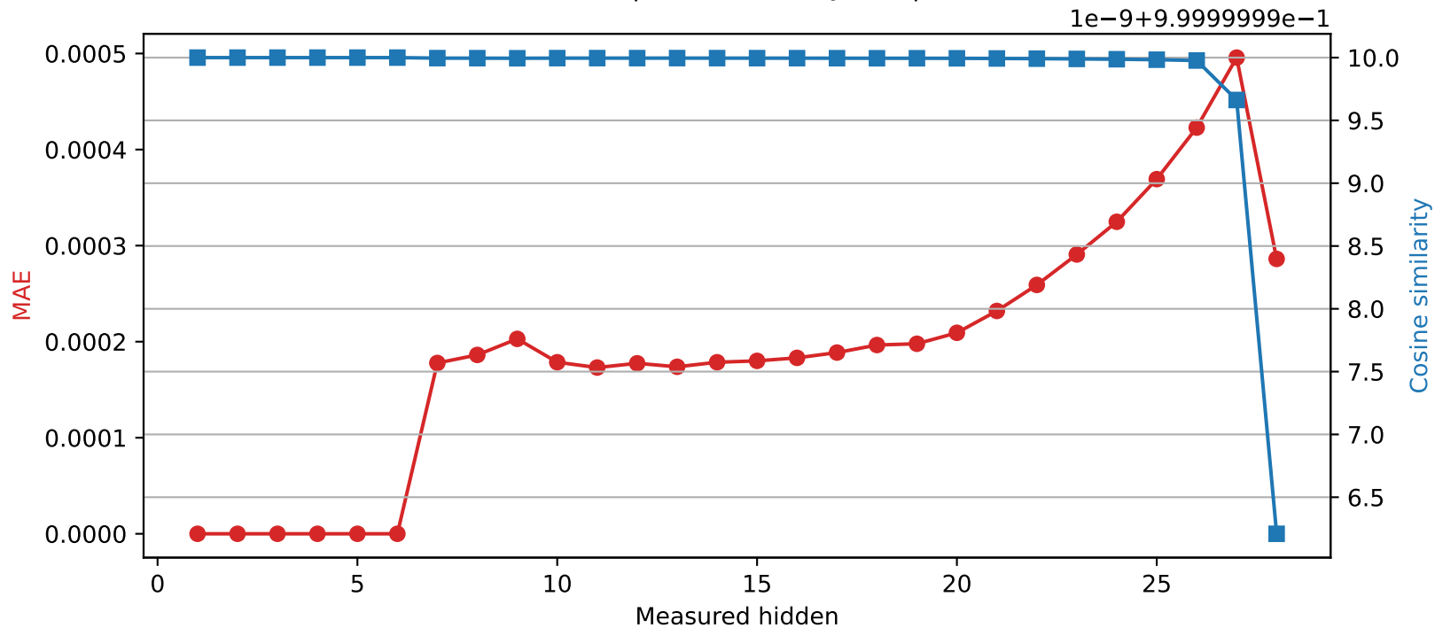
Qwen2.5-7B-Instruct | Quantized layer 6 | float32 → int16
