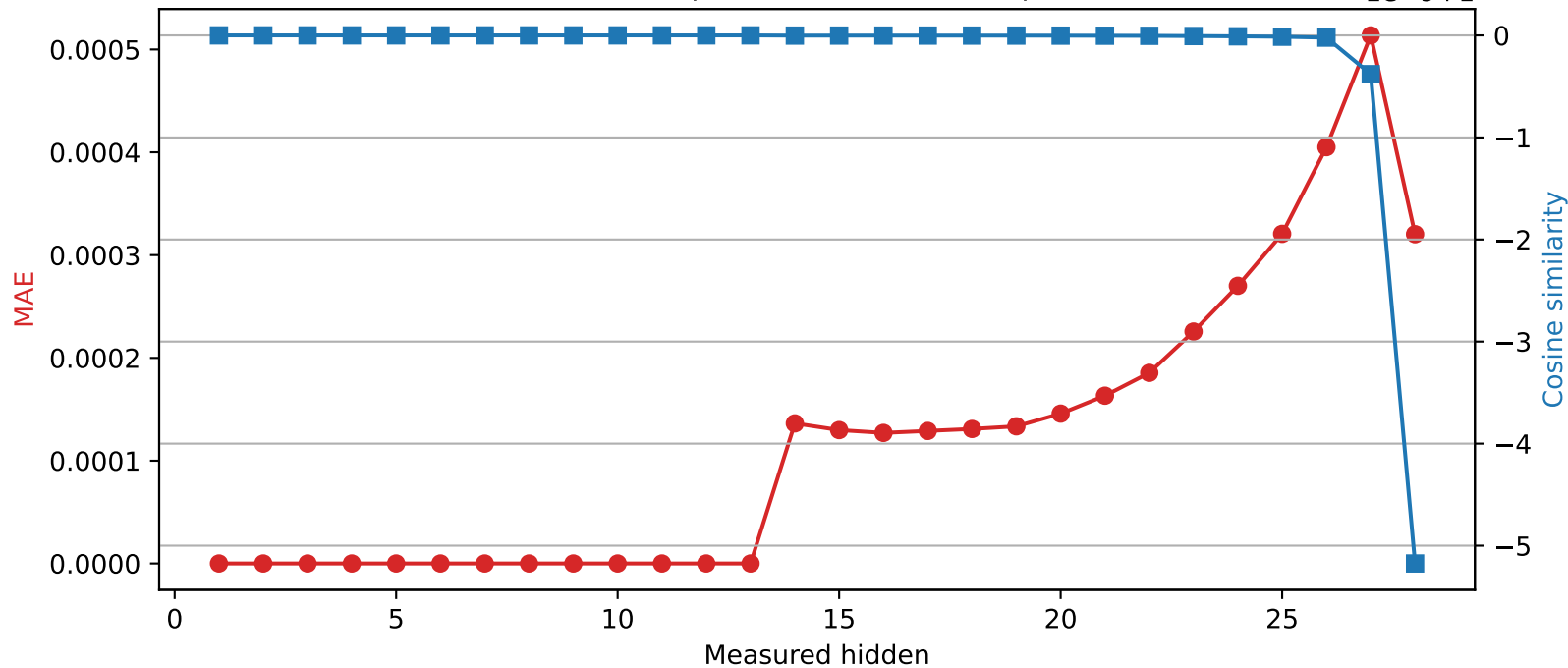
Qwen2.5-7B-Instruct | Quantized layer 13 | float32 \rightarrow int16
